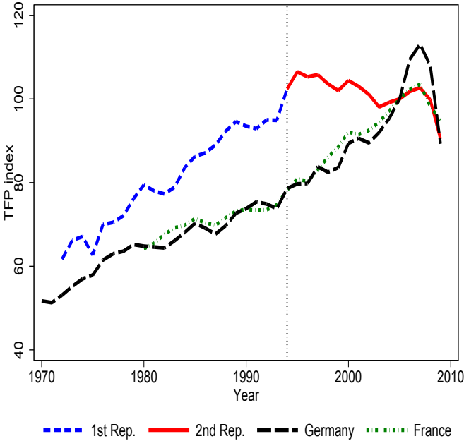
Figure 9: Italy’s TFP
