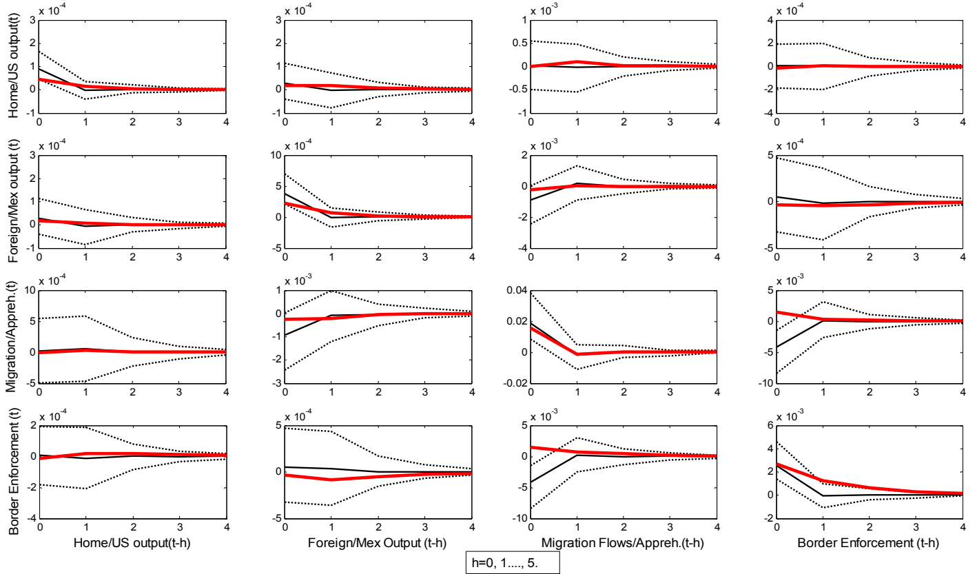
Figure 4. Autocovariance functions
