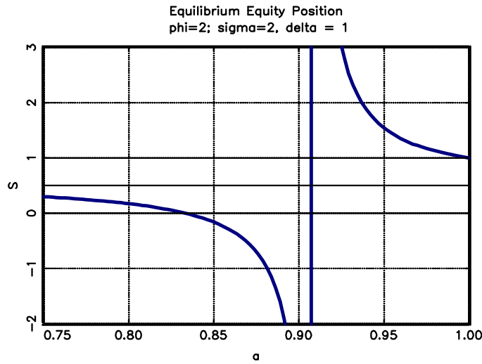
Figure 1: The instability of optimal equity position as a function of preference parameters.
