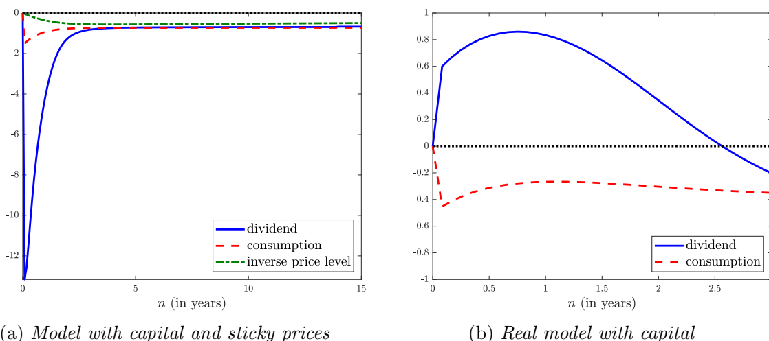
Figure 4: Model with capital: Generalized impulse response to -1 standard deviation productivity shock, starting from the ergodic mean of the states; percentage changes in cash flows over a given horizon
