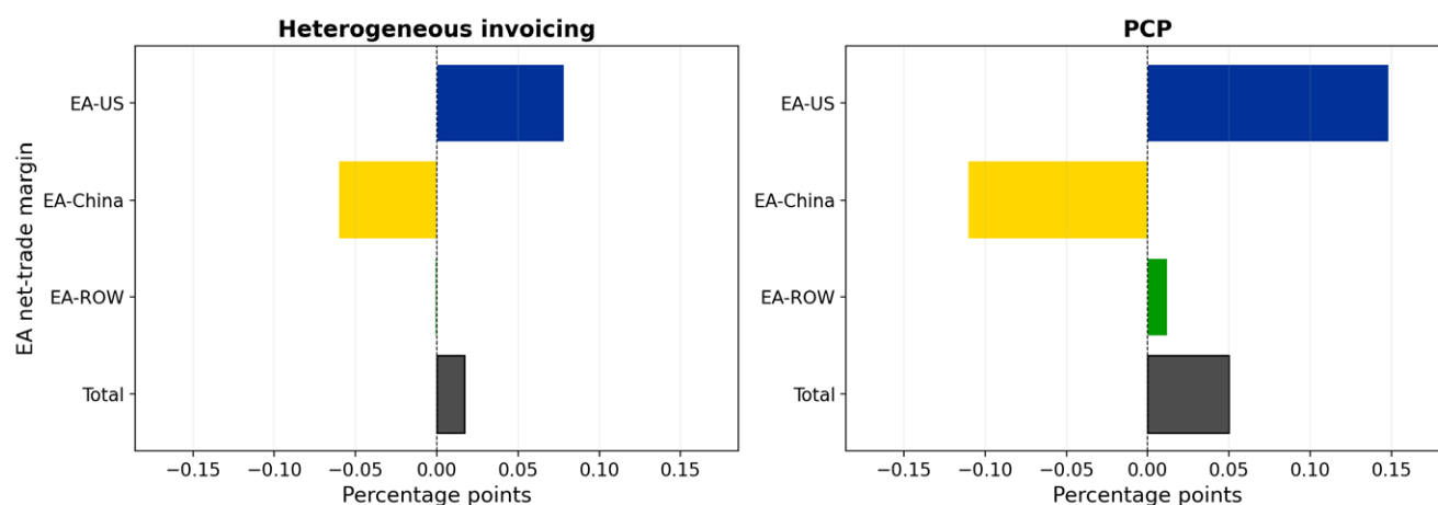
Figure 5: Euro-area Net-trade Margins by Invoicing Regime
