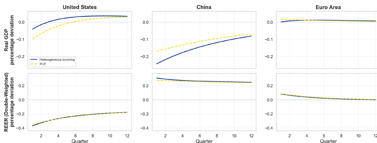
Figure 4: Real Effective Exchange Rates by Invoicing Regime
