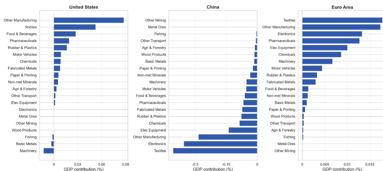
Figure 8: Sectoral Contributions to GDP
