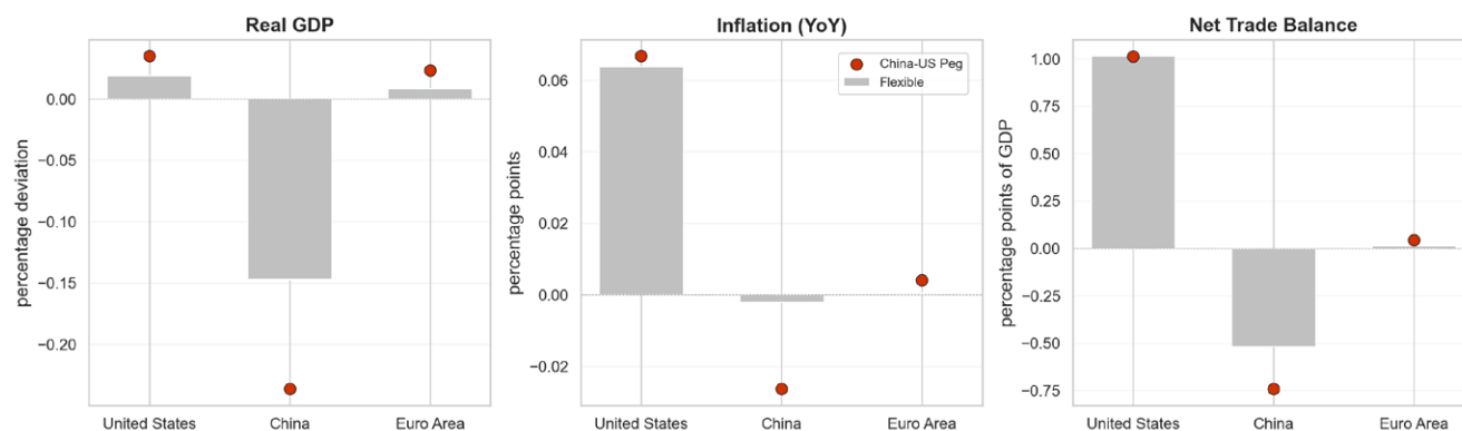
Figure 7: Exchange-rate Regime Average Responses
