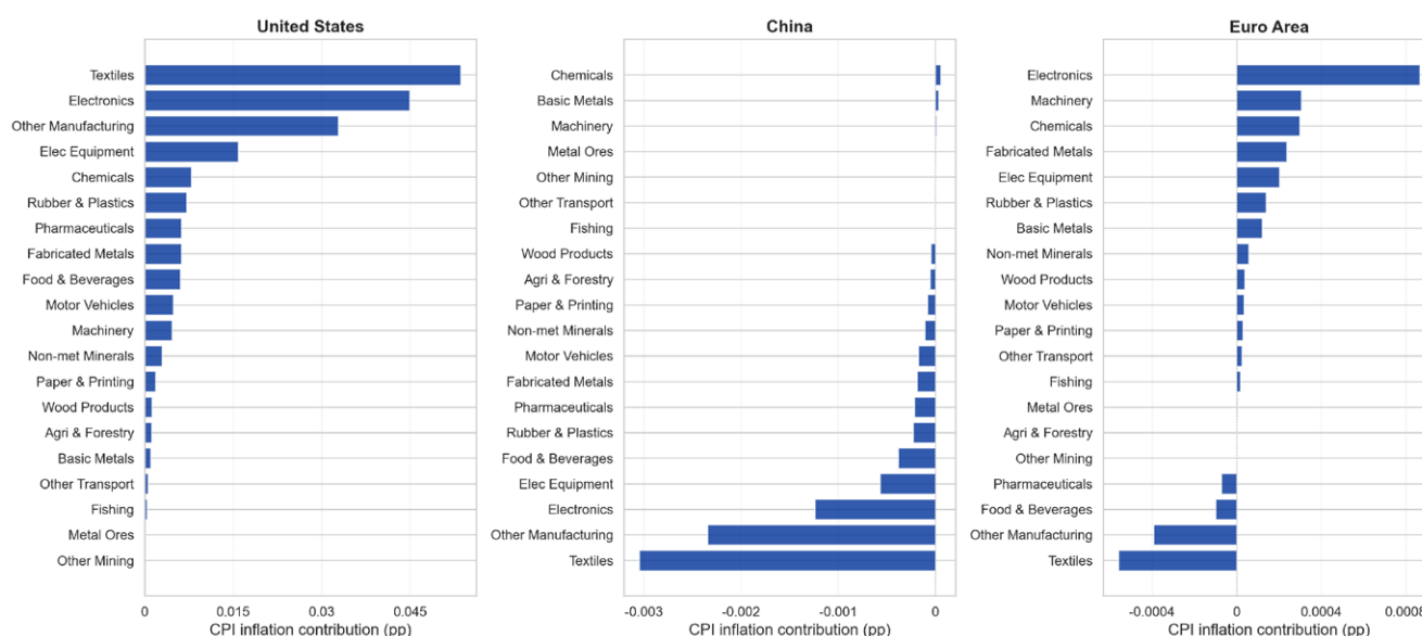
Figure 9: Sectoral Contributions to Inflation
