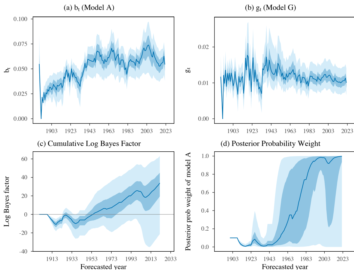
Figure 13: Autoregressive Specification
