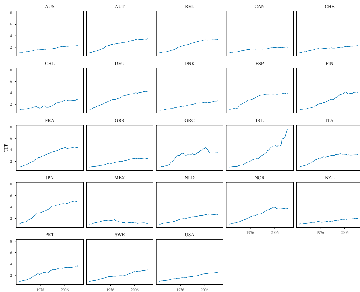
Figure C9: TFP Levels
