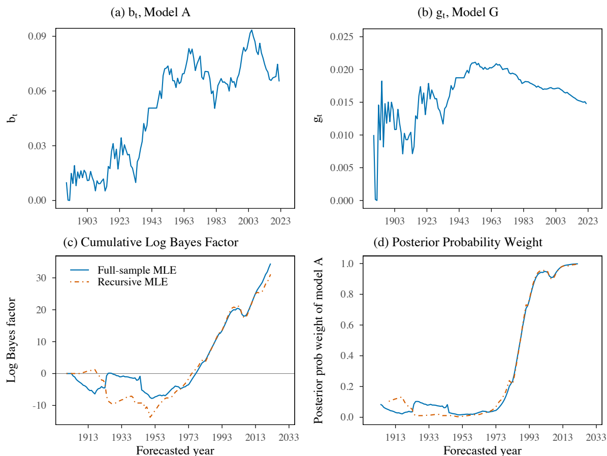
Figure 11: MLE Filtered States and Model Evaluation
