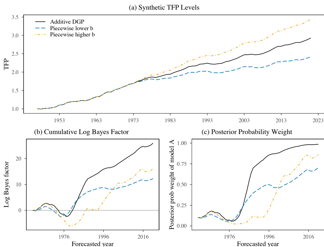
Figure A1: Simulated Additive Data and Model Fit
