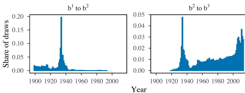
(b) Estimated Break Dates
