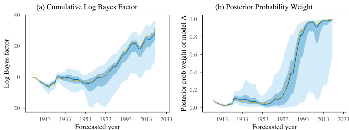
Figure 6: Log Bayes Factor and Posterior Model Weight
