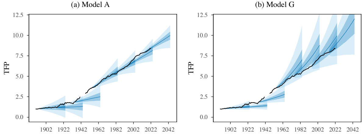
Figure 5: TFP Level and Forecasts
