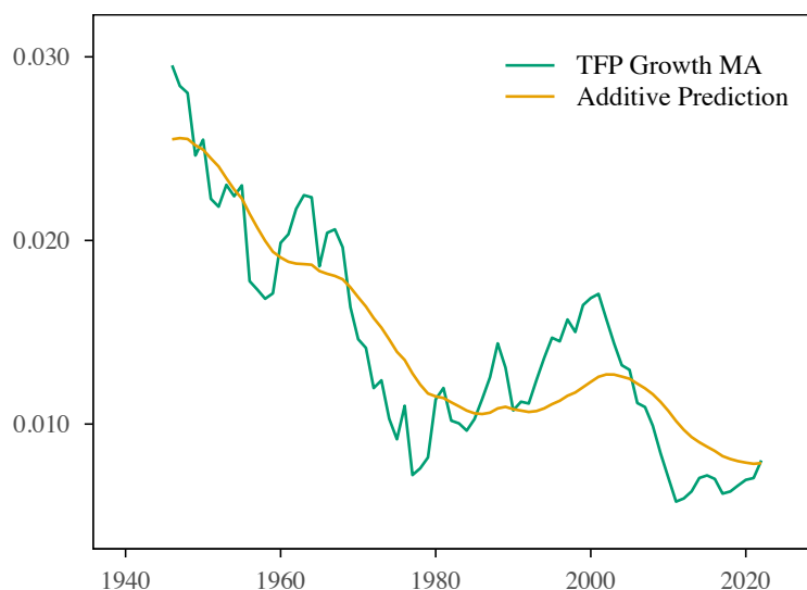
Figure 2: Predicted TFP Slowdown
