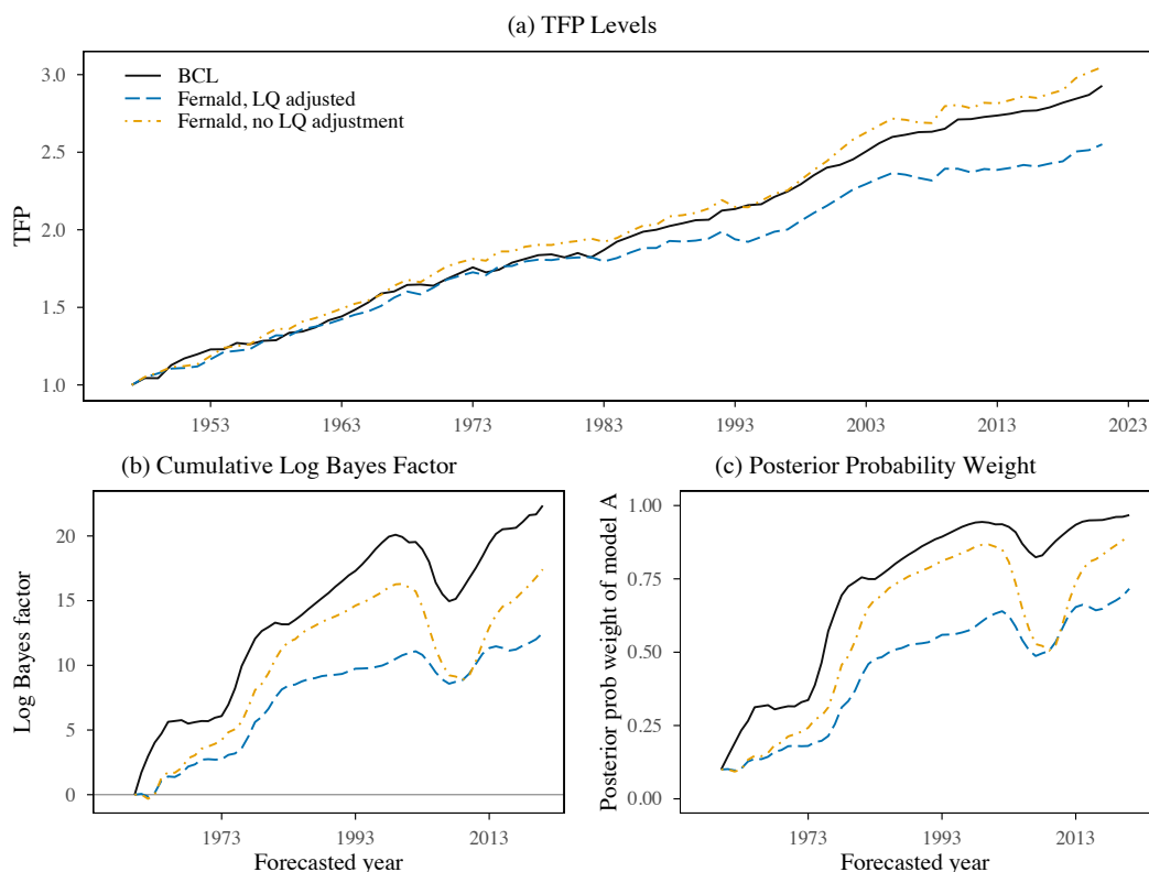
Figure 7: Alternative TFP Measures and Model Fit
