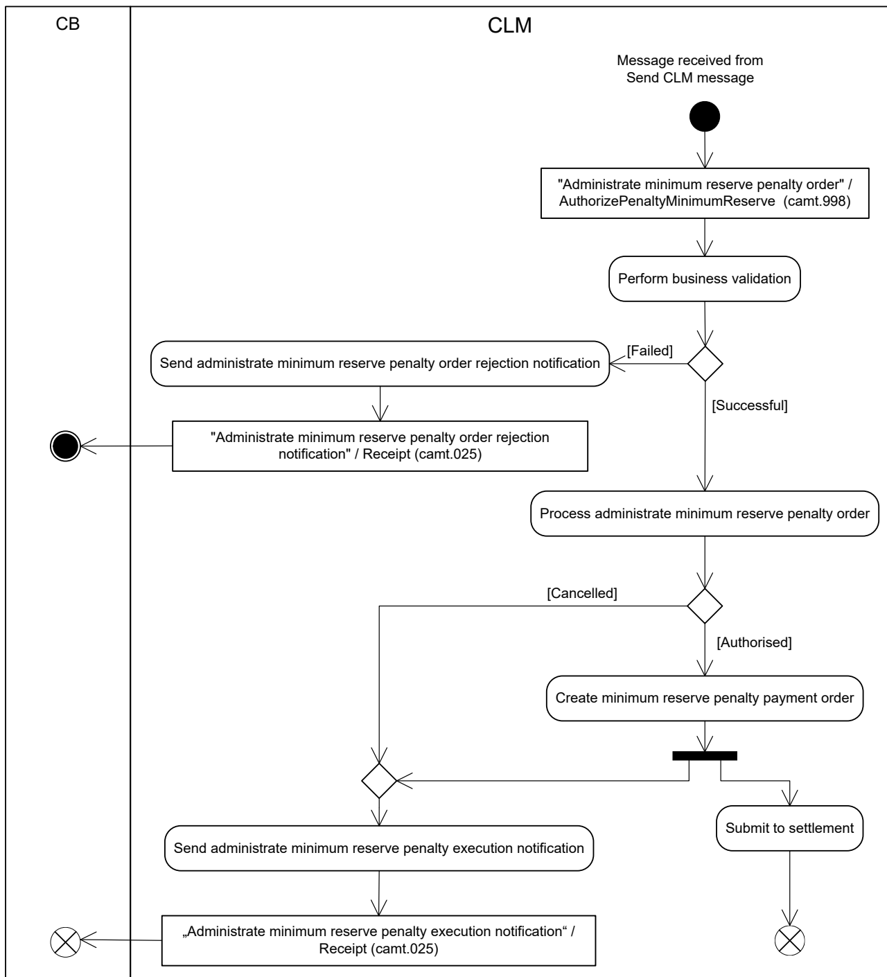
Figure 81 - Administrate minimum reserve penalty order
