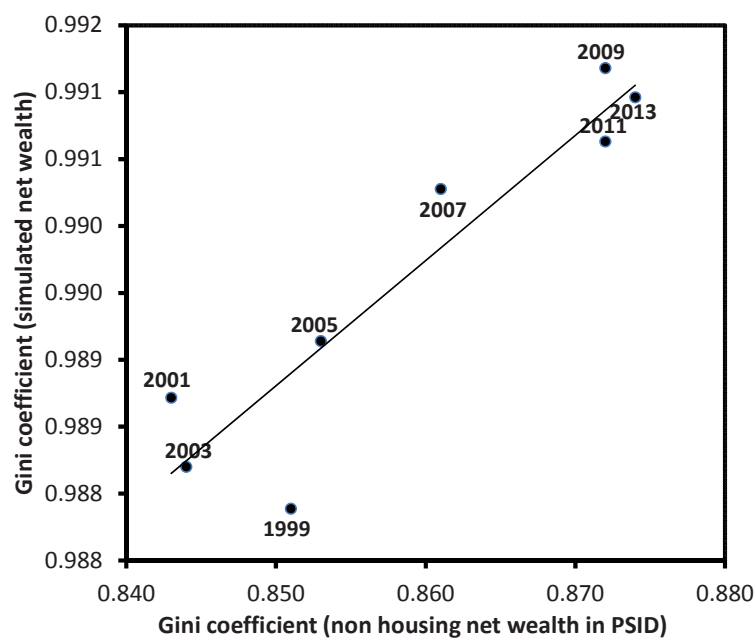
Figure 11: GINI COEFFICIENT
