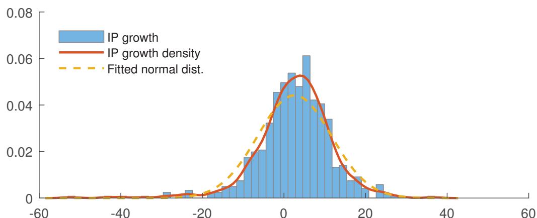
Figure 13: Histogram of annualized US IP growth between March 1960 and February 2016
