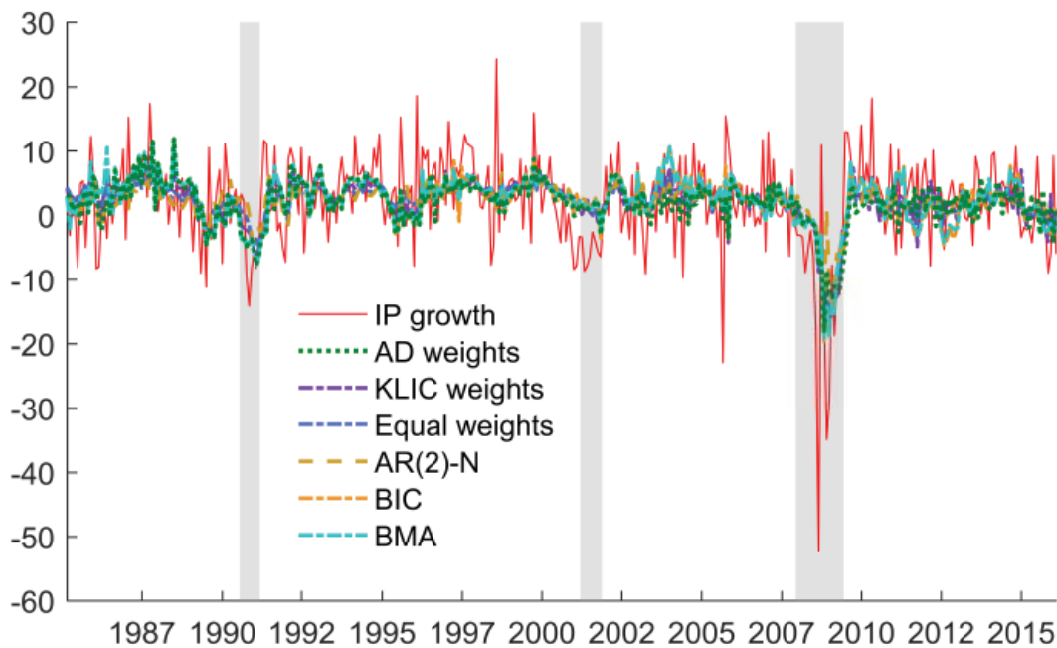
Figure 15: Point forecasts of US industrial production growth
