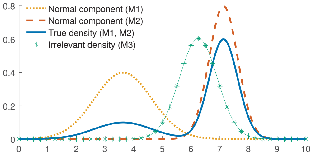
Figure 6: DGP 2 – Comparison of predictive densities
