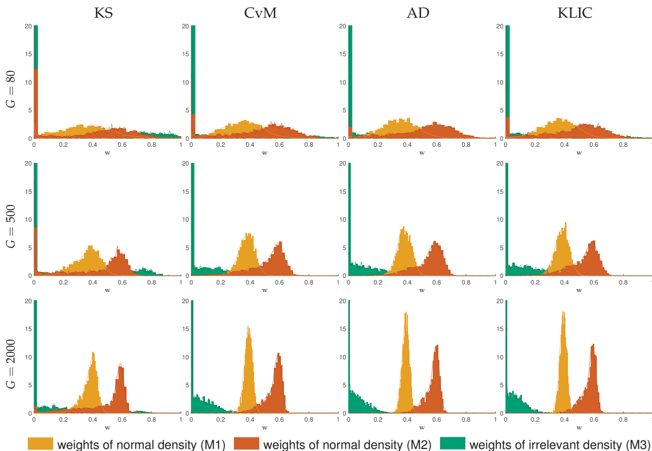
Figure 9: Monte Carlo results for DGP 1b, true parameter vector w^* = (0.4, 0.6, 0)'
