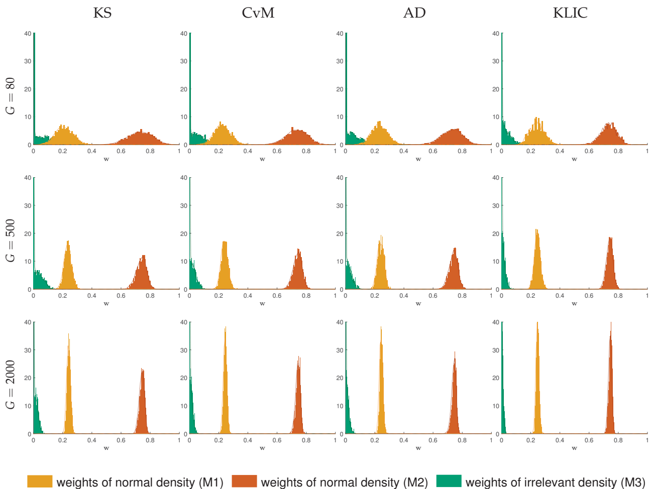
Figure 10: Monte Carlo results for DGP 2, true parameter vector w^* = (0.25, 0.75, 0)'
