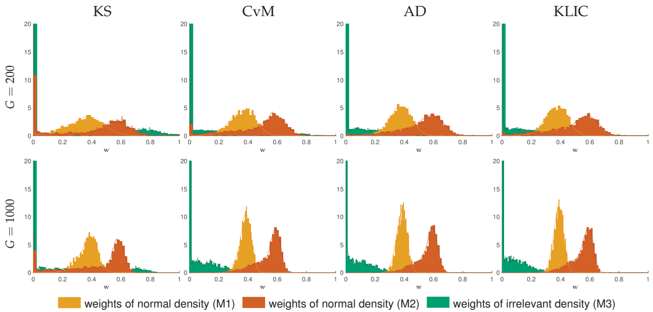
Figure D.1: Additional Monte Carlo results for DGP 1a, true parameter vector w^* = (0.4, 0.6, 0)'
