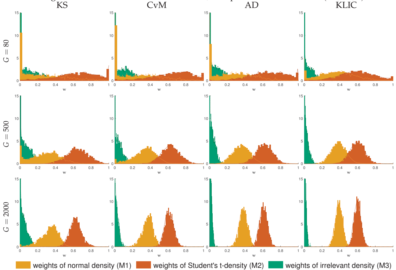
Figure 11: Monte Carlo results for DGP 3, true parameter vector w^* = (0.4, 0.6, 0)'
