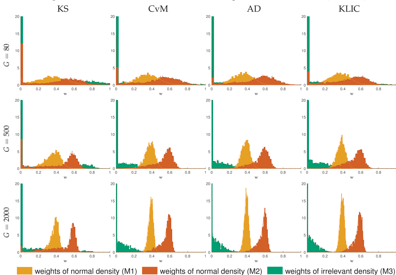
Figure 8: Monte Carlo results for DGP 1a, true parameter vector w^* = (0.4, 0.6, 0)'
