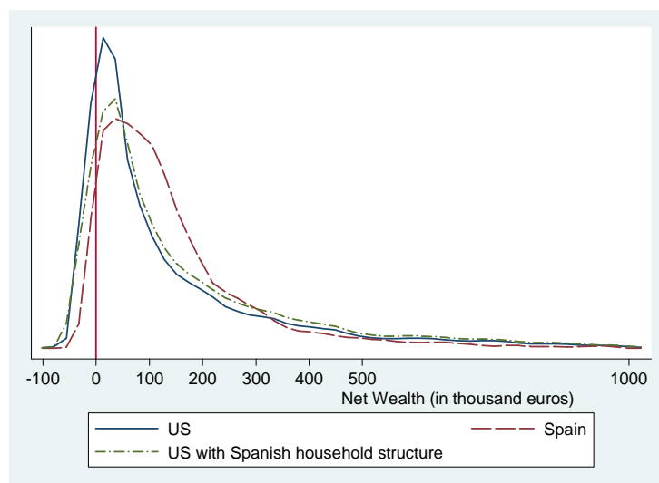
Figure 1A: Estimated densities
