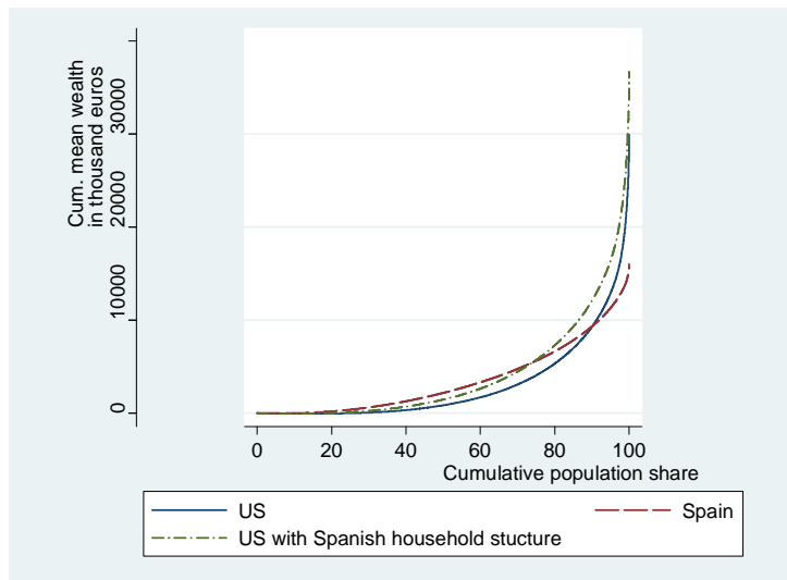
Figure 4: Generalized Lorenz curves
