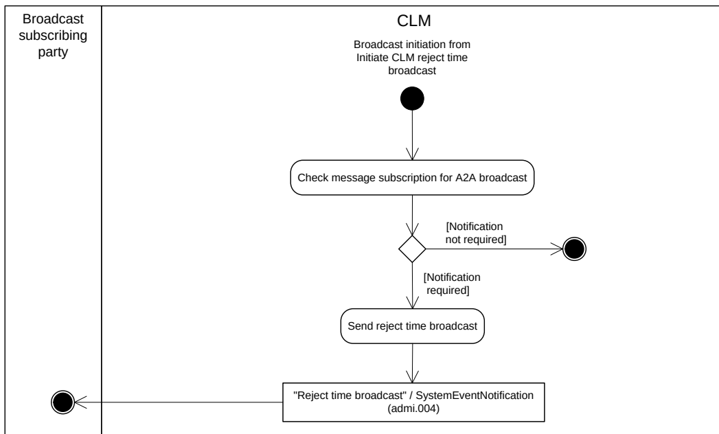
Figure 57 - Process CLM reject time broadcast
