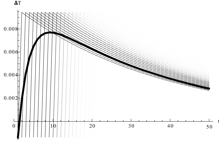
Figure 26: Increase in taxes a result of renegeing on optimal policy when the duration of government debt is 16 quarters. Each line represents the response of the long-term interest rate when the efficient rate of interest returns to its steady-state in that period.
