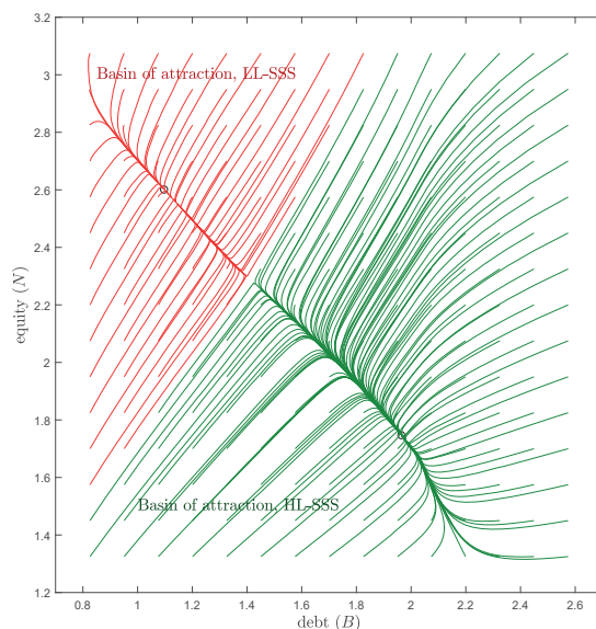
Figure 7: Convergence paths.
