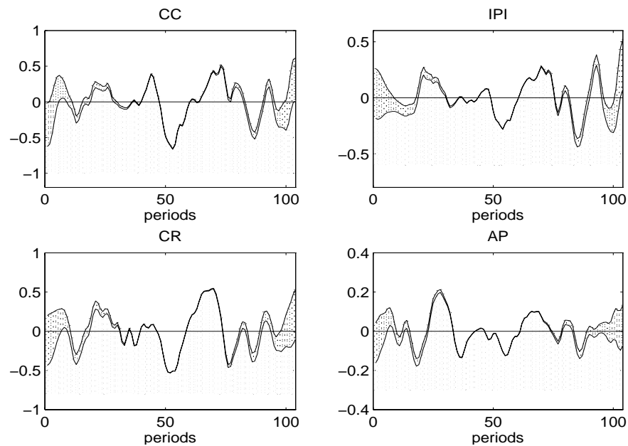
Fig. 22. 95% CI for HP cycle (based on revisions)
