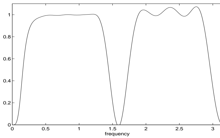
Fig. 6. Squared gain: Convolution of HP and X11 filters
