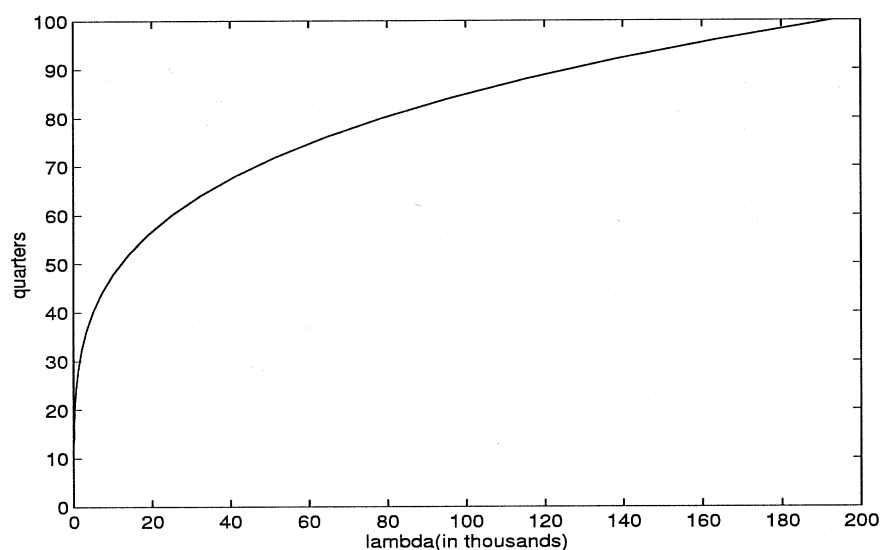
Fig. 10. Period of cycle as a function of lambda
