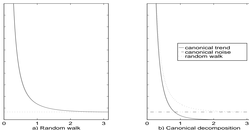
Figure 3.6. Canonical Decomposition of a Random Walk
