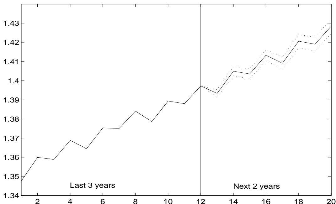
Figure 3.3 Forecasts and 90% confidence interval
