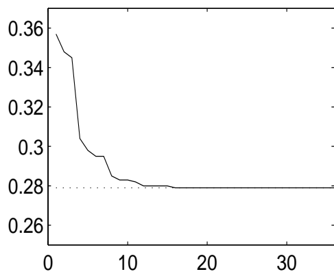
c) Seasonal component
