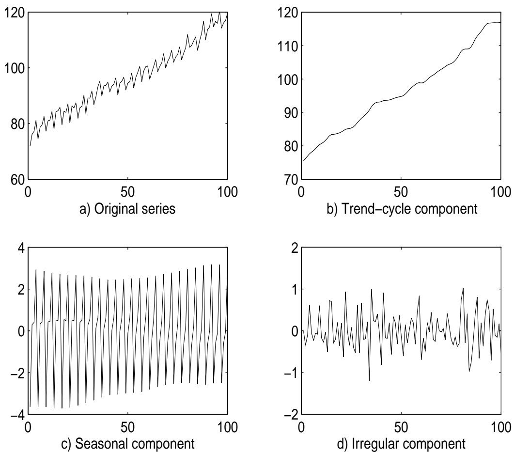
Figure 3.10. Series and Estimated Components
