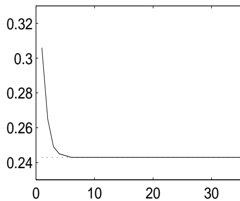
b) Trend-cycle component
