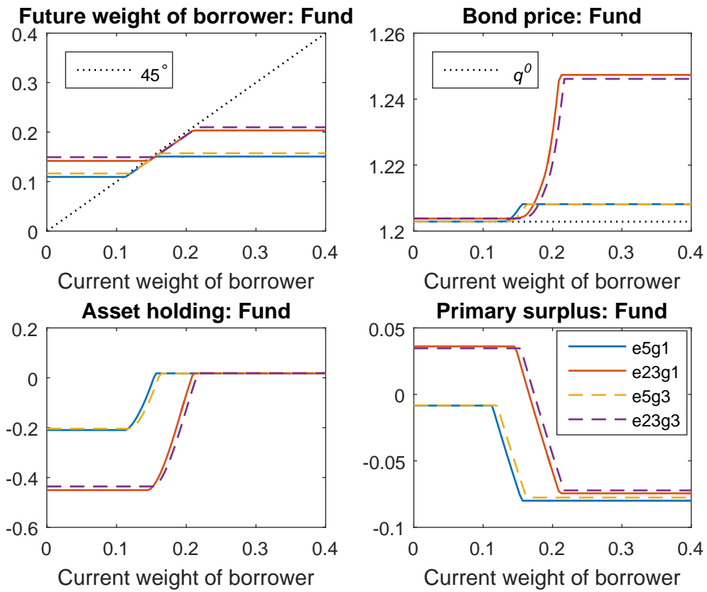
Figure 3: FSF policy functions: Pareto weights and assets.
