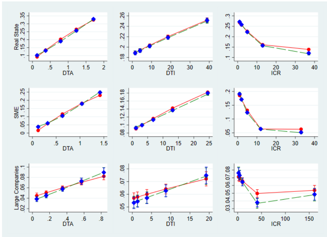
Figure A5. Predictive margins: linear probability model Vs Logit and Probit
