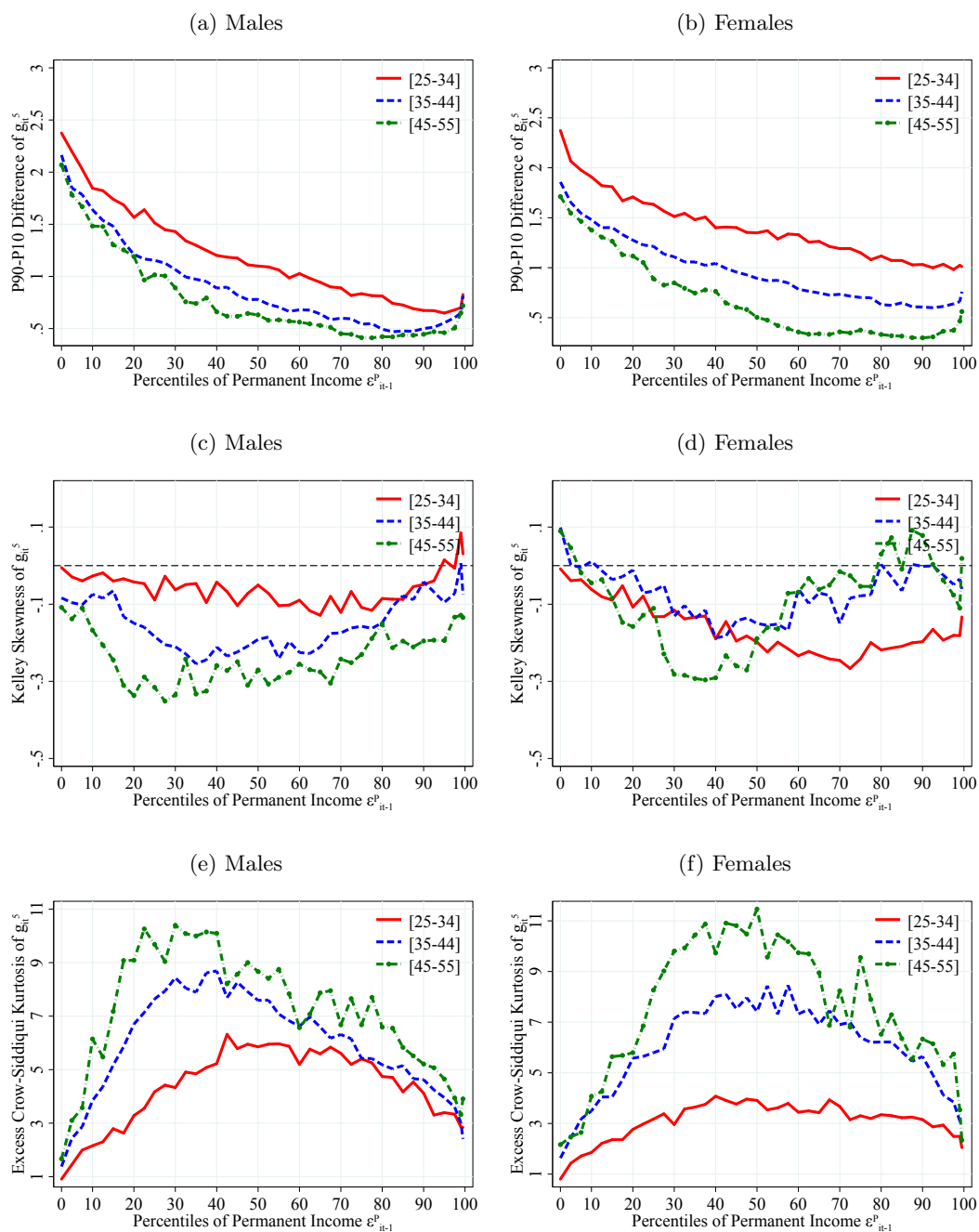
Figure F20: Dispersion, skewness and kurtosis of five-year earnings changes
