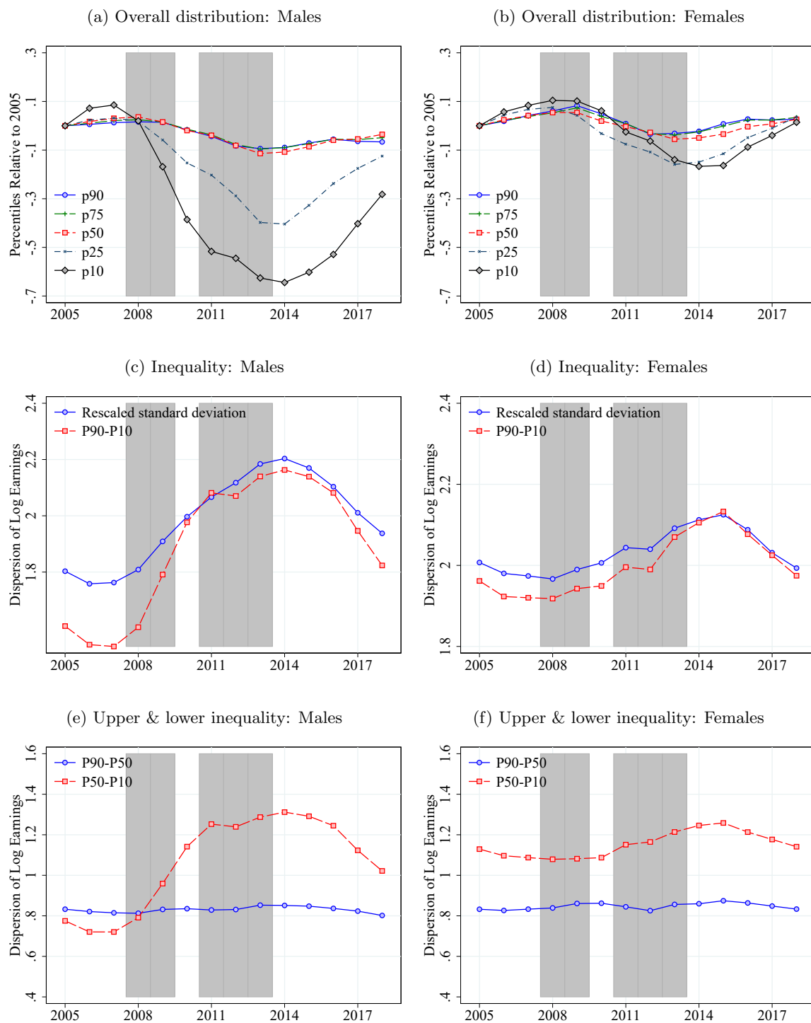
Figure F8: Evolution of income percentiles and inequality, earnings & unemployment benefits
