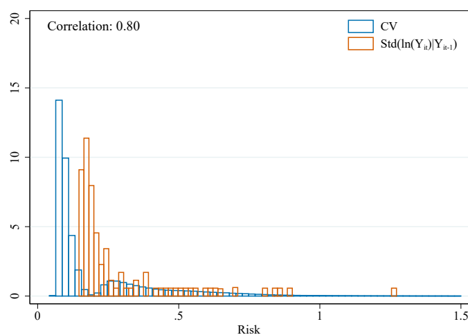
Figure 12: Comparing CV and standard deviation
