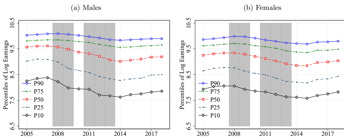
Figure F25: Overall distribution of workers at age 25
