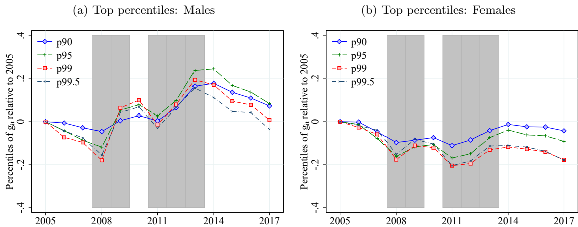
Figure F14: Top percentiles of one-year changes in log earnings
