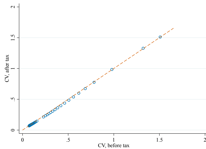
Figure G4: Quantile-quantile plot of before-tax and after-tax CV
