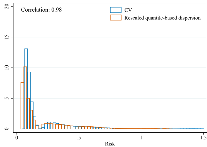
Figure G16: Comparing CV and quantile-based dispersion
