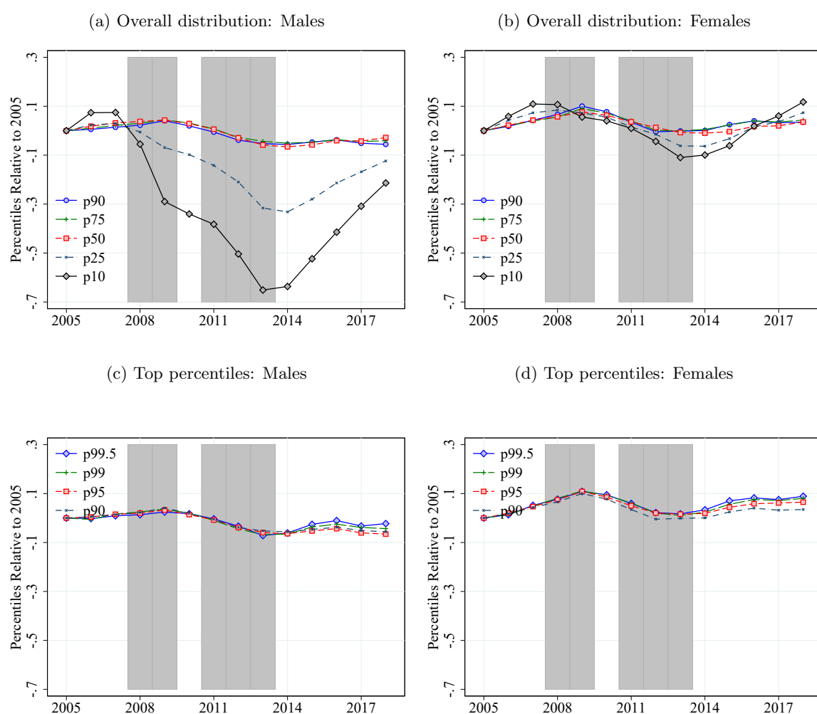
Figure 2: Percentiles of the distribution of log annual earnings
