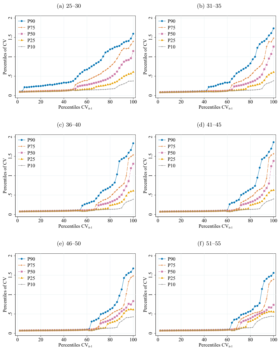
Figure G2: CV persistence, by age
