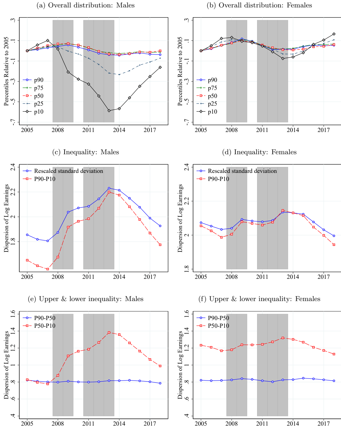
Figure F9: Evolution of earnings percentiles and inequality, no immigrants
