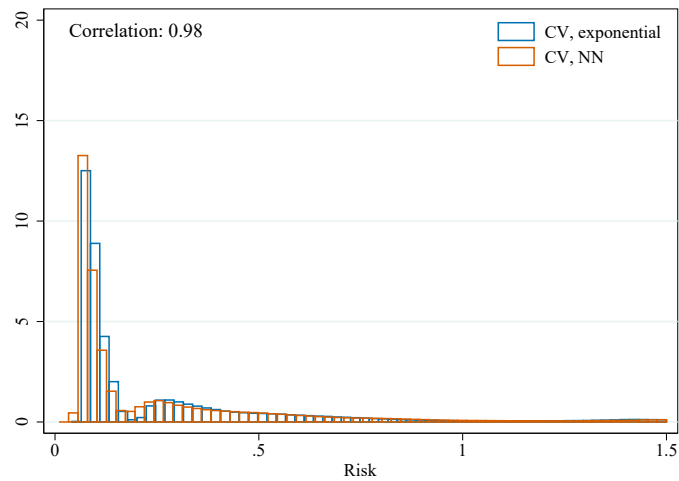
Figure G8: Two specifications of CV, exponential and neural network
